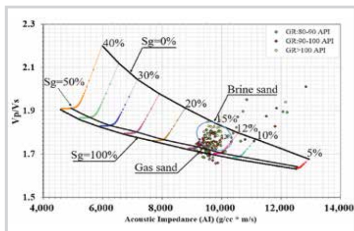
Figure 16. The RPT constructed in this study for MMS.
